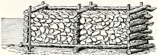
CRIB OF STONE AND BRICK.
